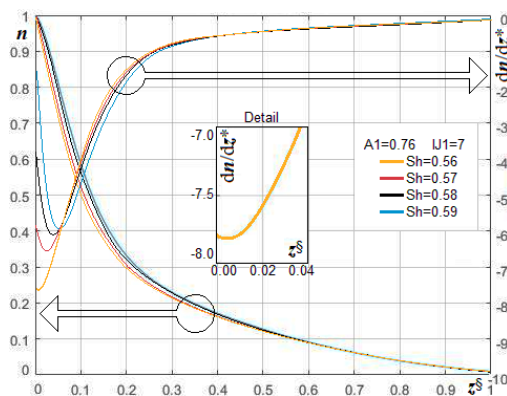
Fig. 5. Curves n and dn/dz^* for A_1=0.76 , IJ_1=7 , variable Sh with maximum slopes of n for z^s \neq 0 .
