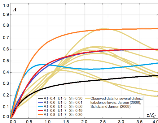
Fig. 7. RSW A -profiles for several sets of parameters, and observed A -profiles for various agitation conditions
