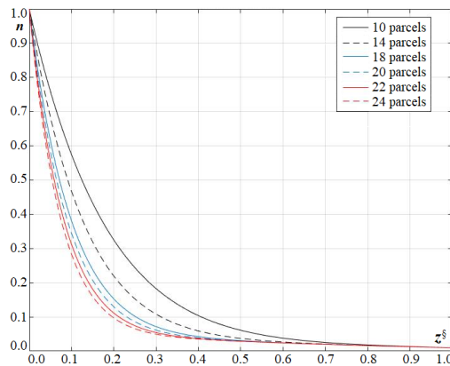
Fig. 9. Effect of number of parcels of the Taylor series on the n -profile for A_1=0.6 , IJ_1=7 , Sh=0.1 .
