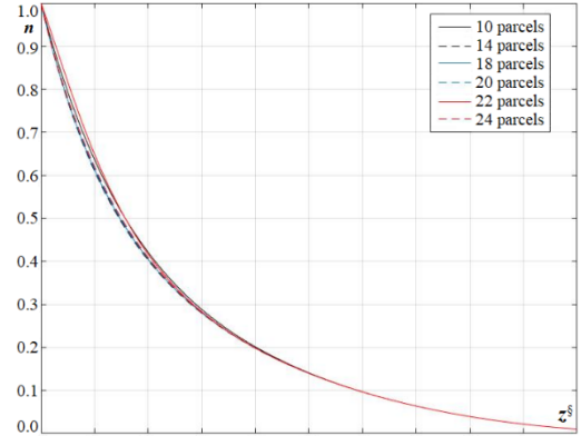
Fig. 12. Effect of number of parcels of the Taylor series on the n -profile for A_1=0.6 , IJ_1=7 , Sh=0.49 .
