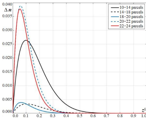
Fig. 13. Differences between successive n -profiles for A_1=0.6 , IJ_1=7 , Sh=0.49 .
