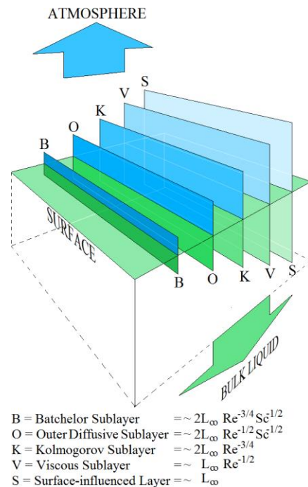
Fig. 1. BOKVS-BOKVS layers at gas-liquid interfaces. The heights of the vertical planes above and below the surface indicate thicknesses of the gaseous and liquid layers, respectively.
