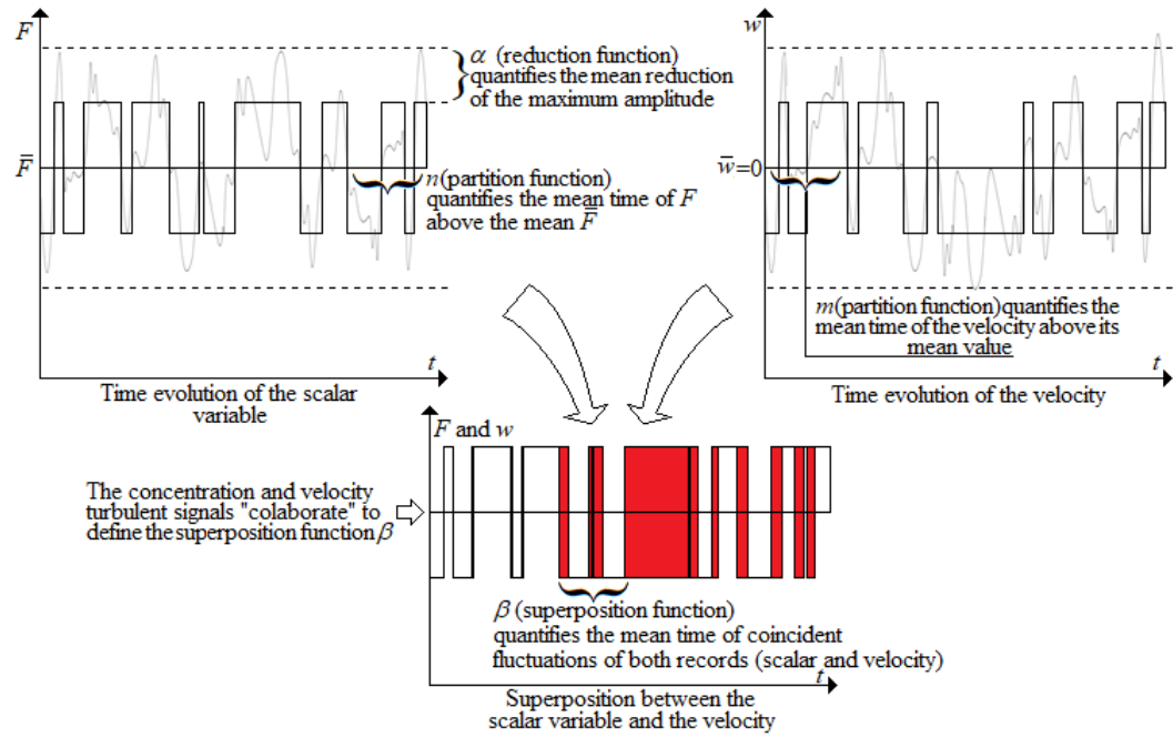
Fig. 2. The RSW method used to model concentration and velocity signals to square waves, keeping the mean values of the original signals. The proposed statistical functions have clear physical meanings
