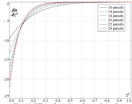
Fig. 11. Effect of number of parcels on the profile of dn/dz^s for A_1=0.6 , IJ_1=7 , Sh=0.1 .
