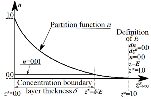
Fig. 3. Boundary conditions that define E and \delta , conditioned by the partition function n .
