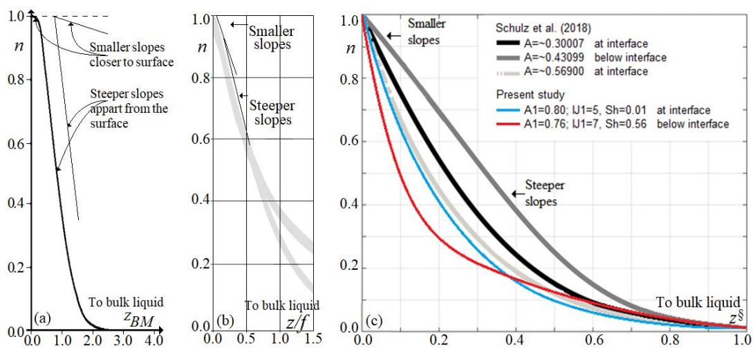
Fig. 4. n profiles: a) Laminar flows adapted from Boyadjiev and Mitev (1977); b) Envelope of measured data of Friedl (2013), turbulent flows; c) RSW results: black and gray tones from literature for steady state and constant A . Colored red and blue profiles are results of the present study.
