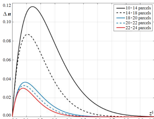
Fig. 10. Differences between successive n -profiles for A_1=0.6 , IJ_1=7 , Sh=0.1 .
