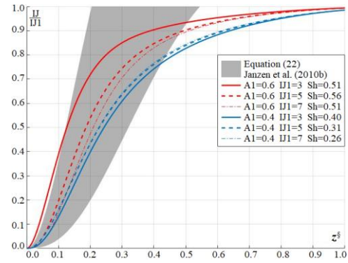
Fig. 8. IJ -profiles for IJ_1=5 , A_1=0.4 and 0.6 . Gray represents Eq. (22) from Janzen et al. (2010b).
