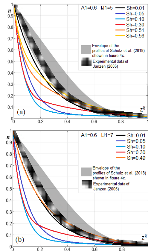
Fig. 6. n curves for A_1=0.6 ; a) IJ_1=5 , variable Sh ; b) IJ_1=7 , and Sh=0.49 close to the observations.
